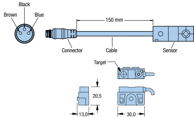
Sensor / Bracket Detail
