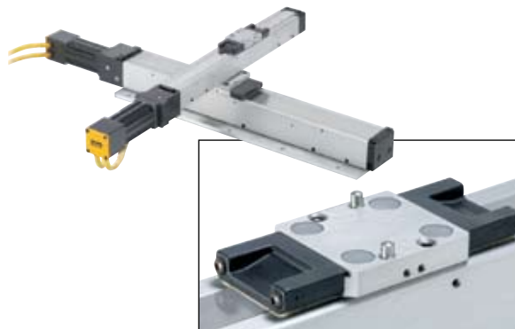
Two locating dowel pins shown in carriage
